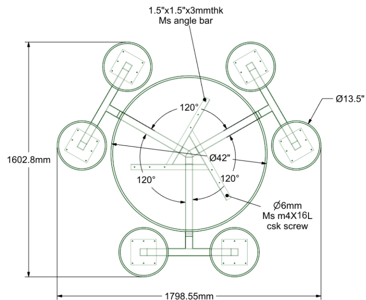
TOP VIEW (HIDDEN LINE)
