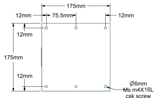
TOP VIEW MS PLATE
