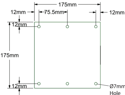
FRONT VIEW (5MMTHK MS PLATE)
