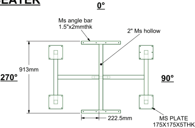
180° TOP VIEW (HIDDEN LINE)
