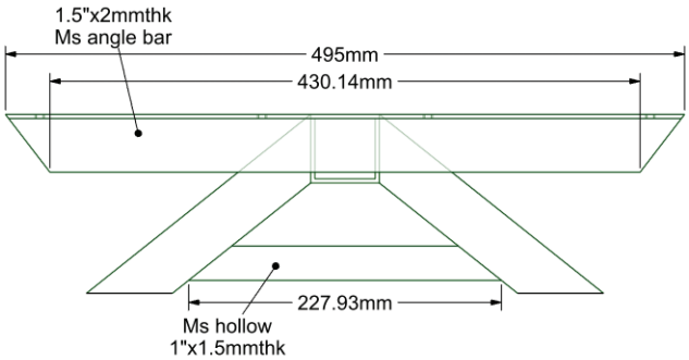
DETAIL B (HIDDEN LINE)
