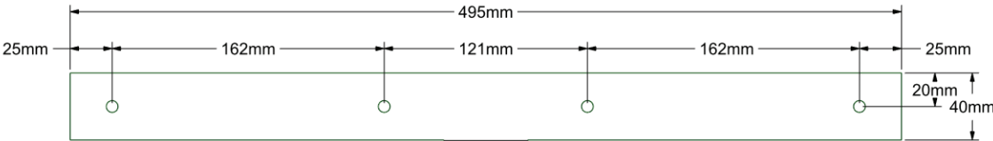
STEEL ANGLE BAR DETAIL
