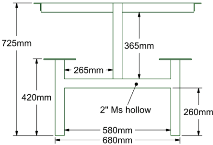
90° VIEW
