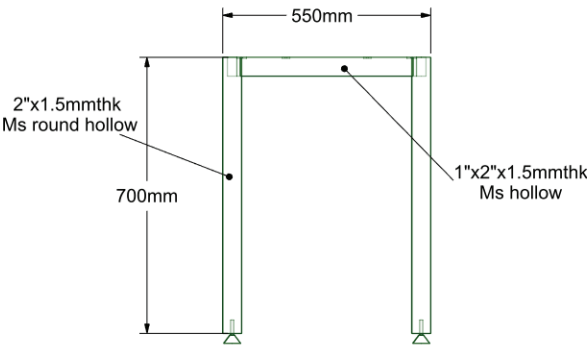
90° VIEW (HIDDEN LINE)
