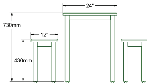
180° VIEW
