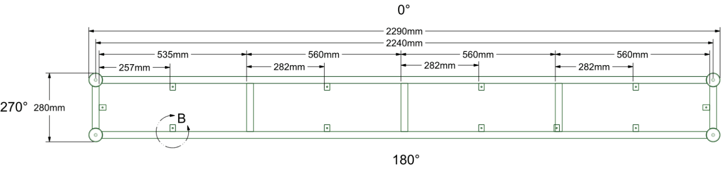
TOP VIEW (HIDDEN LINE)
