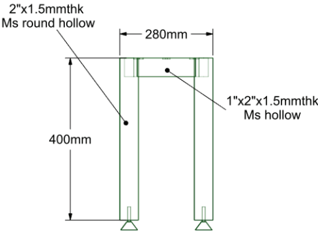
90° VIEW (HIDDEN LINE)
