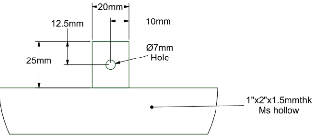
DETAIL B 3MMTHK STEEL BRACKET
